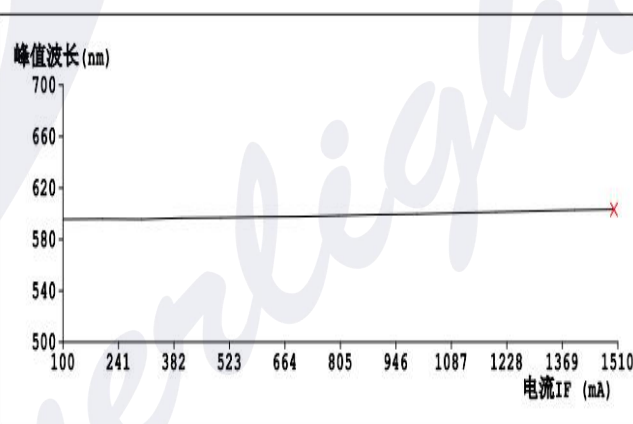
Spectral wavelength
