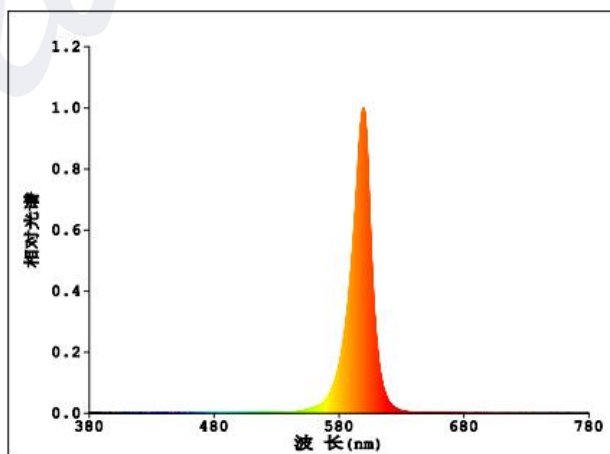
Spectral wavelength
